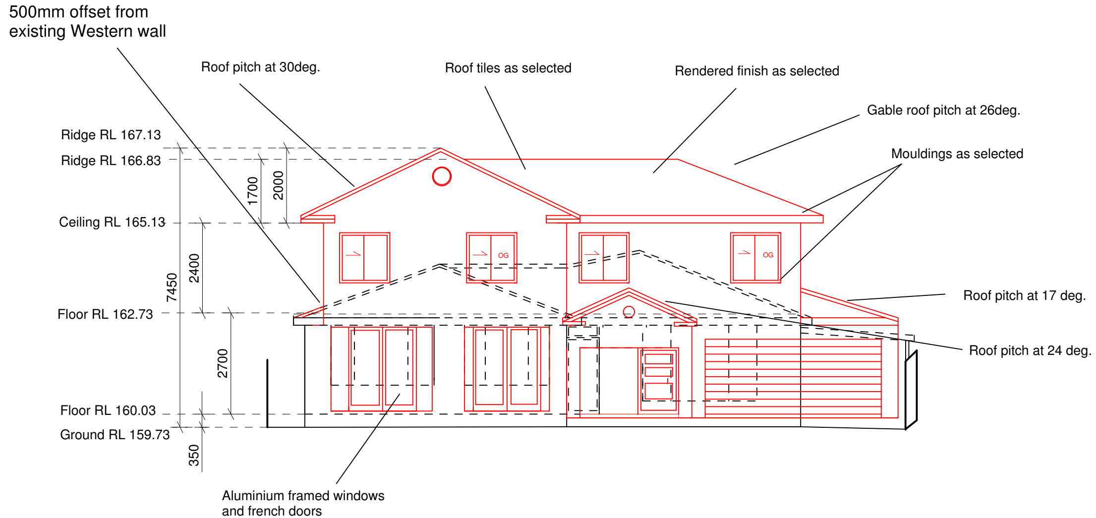
SOUTH ELEVATION
